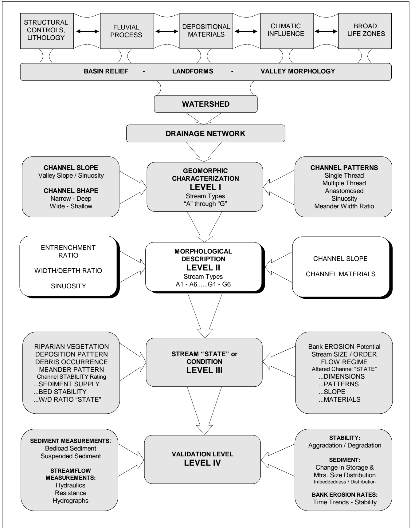
FIGURE 5-1a. The morphological description (Level II) stream classification in relation to the hierarchical river inventory levels
